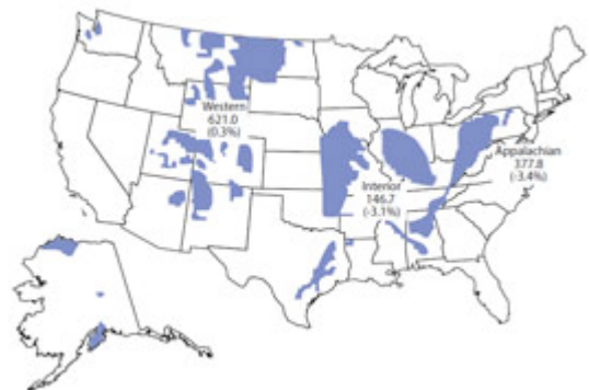
Coal Production in Three Regions, 2007 Millions of Short Tons 1,146.6 Million Short tons
