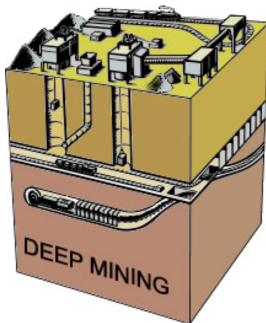
A Typical Deep Mine
